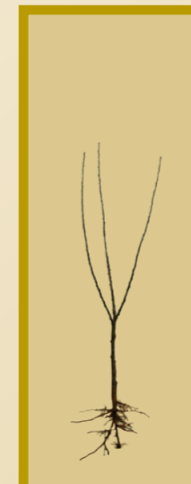
Grafted/occulated rootstock
